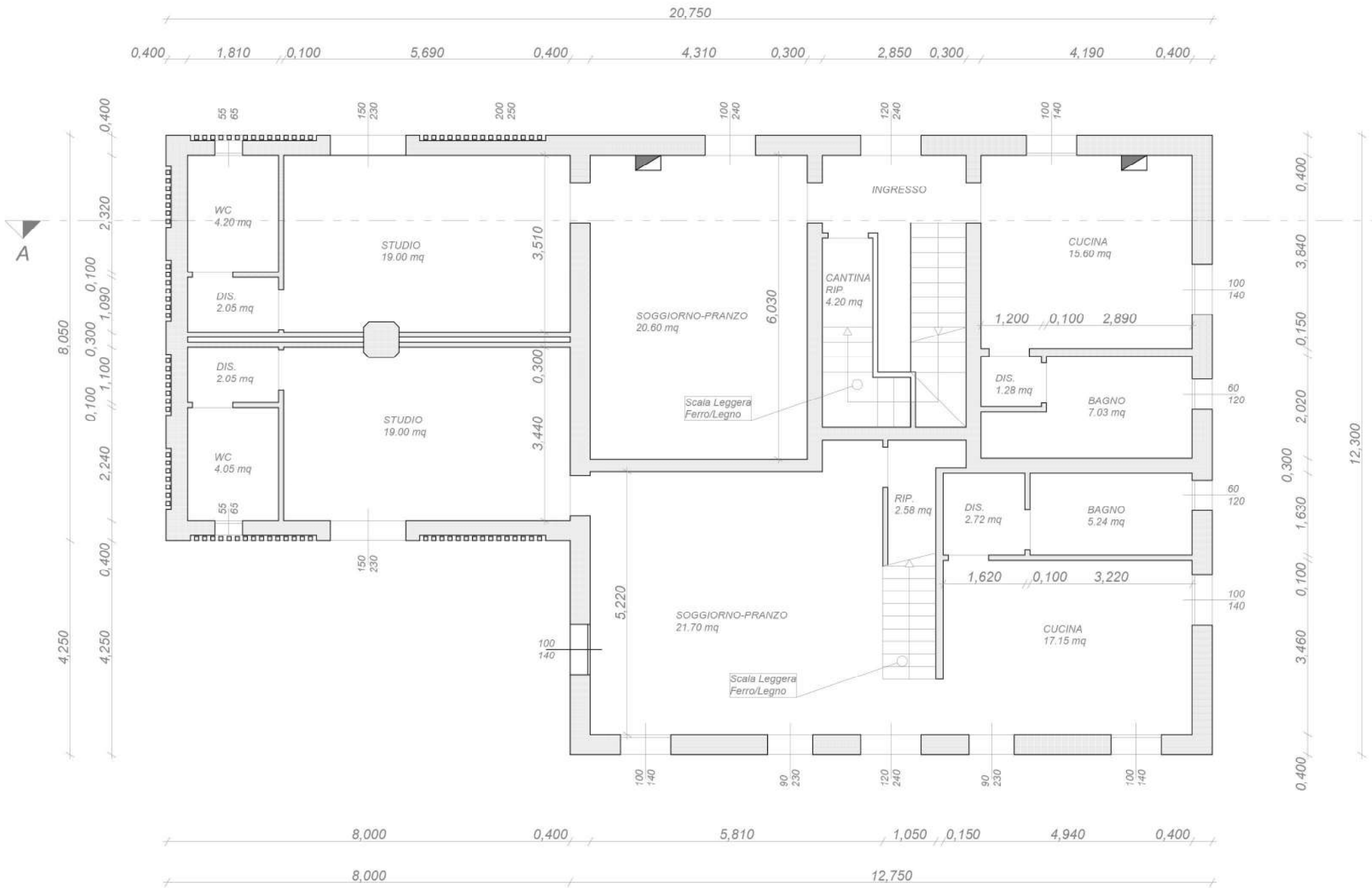
PIANO TERRA
