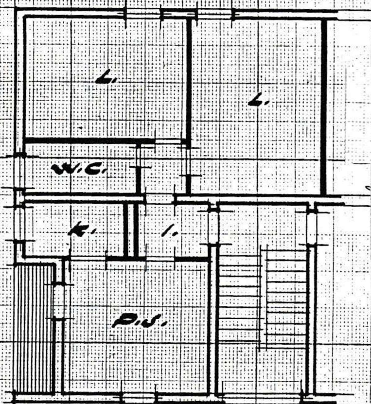
PIANO 2° H=ml. 2.80 SUB. 4
